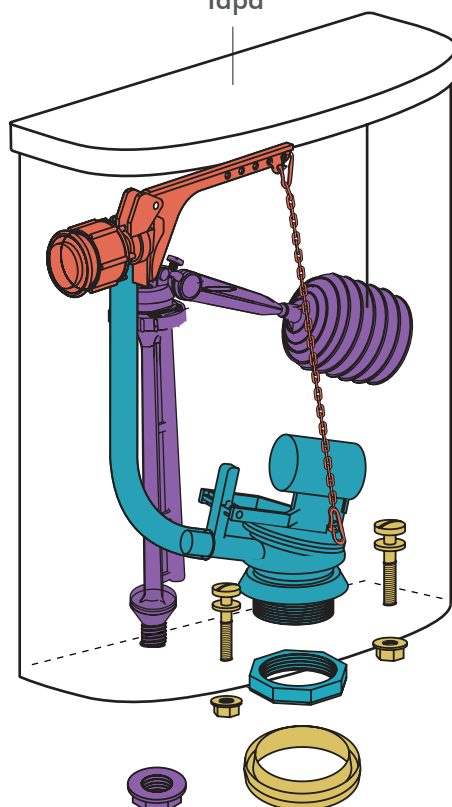
ZTDUR | REP-TD-026-BL Tapa
