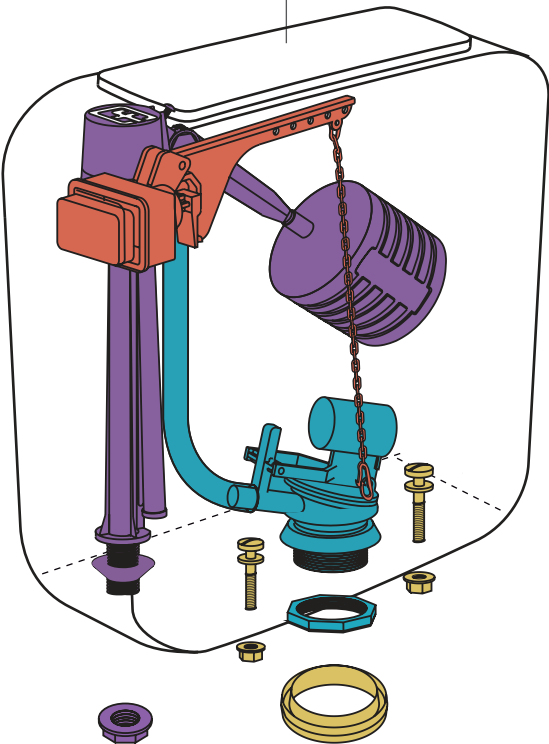
ZTDVM | REP-TD-030-BL Tapa
