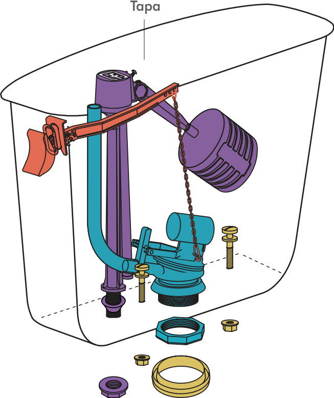
ZTDAP | REP-TD-012-BL Tapa
